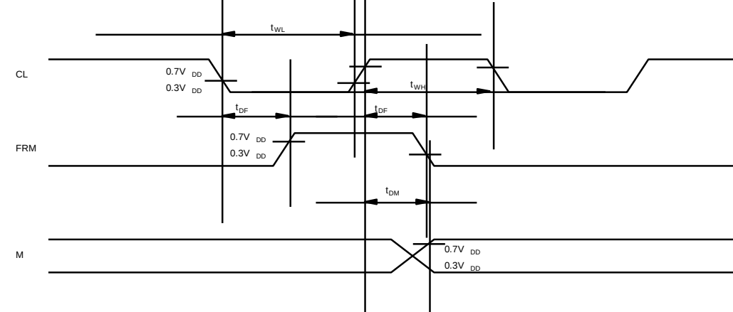
Fig 2. Display control signal waveform
