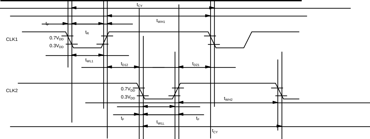
Fig 1. External clock waveform
