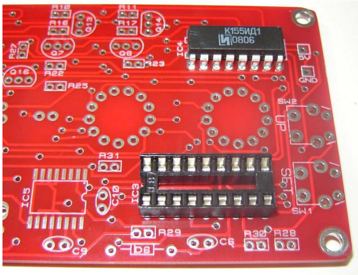
Figure 15: Socket for IC3, and IC4
