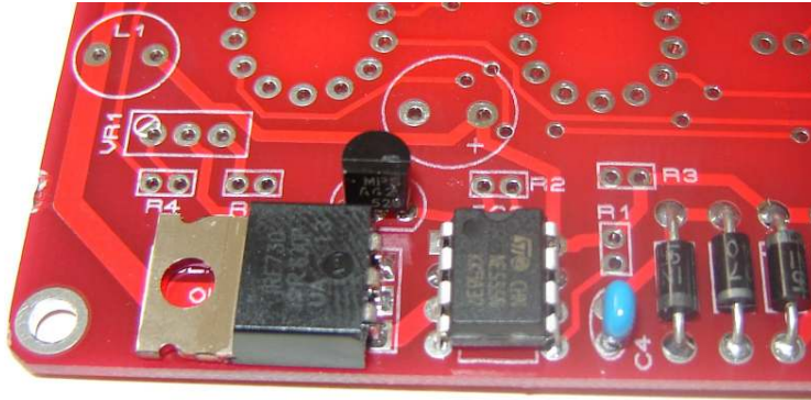
Figure 6: Bending the leads of MOSFET Q2 to lower the profile of the board.
