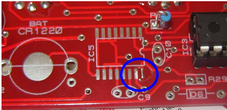
Figure 19: Corner SMD pad wetted with solder
