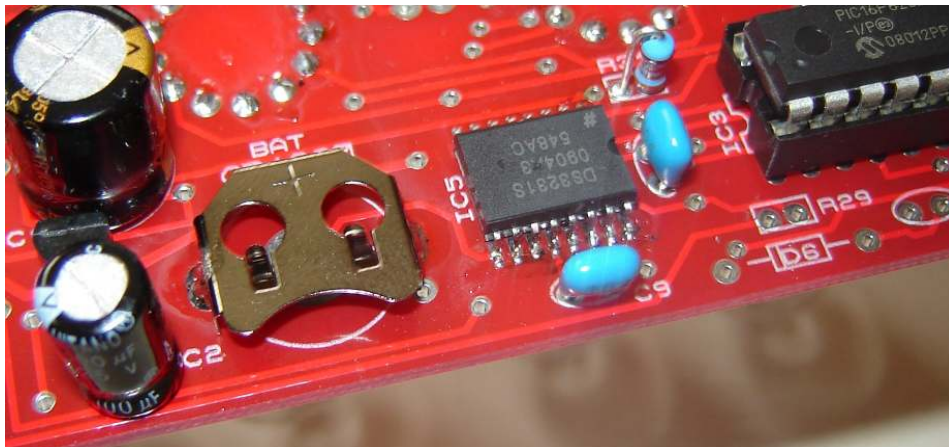
Figure 21: Showing all RTC components: IC5, C9, C10, Lithium Cell Holder
