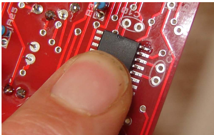
Figure 20: DS3231 placed and held firm
