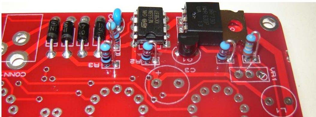
Figure 8: R1 to R5 placed vertically
