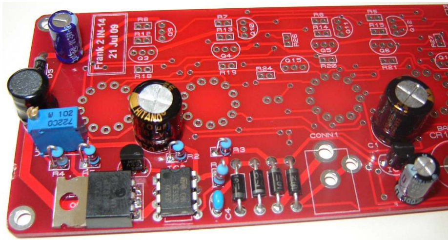
Figure 12: Electrolytic capacitors placed on the PCB
