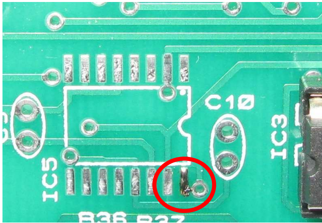
Figure 17: Corner SMD pad wetted with solder
