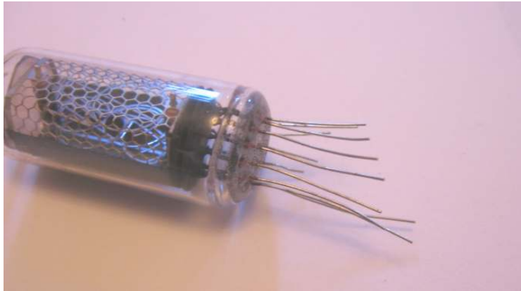
Figure 16: IN-8-2 flying leads trimmed to aid insertion into the PCB
