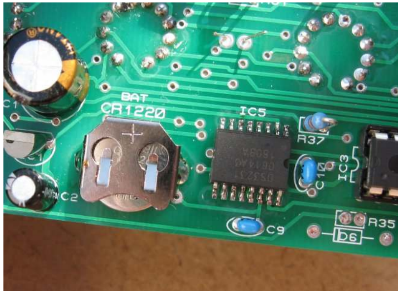
Figure 19: Showing all RTC components: IC5, C9, C10, Lithium Cell
